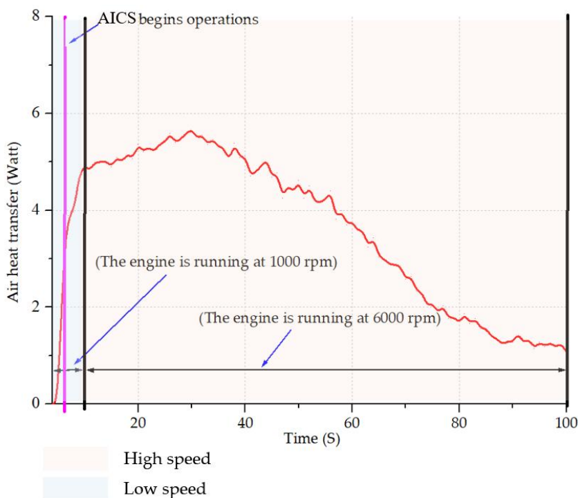
Fig. 12. Air heat transfer
