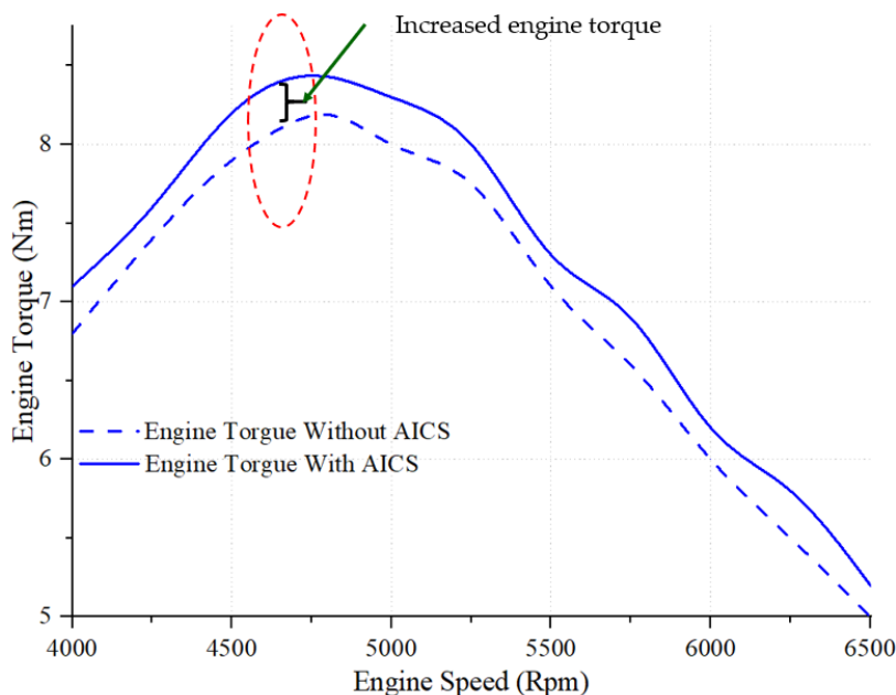
Fig. 6. Increased engine torque when the ambient air temperature is hot
