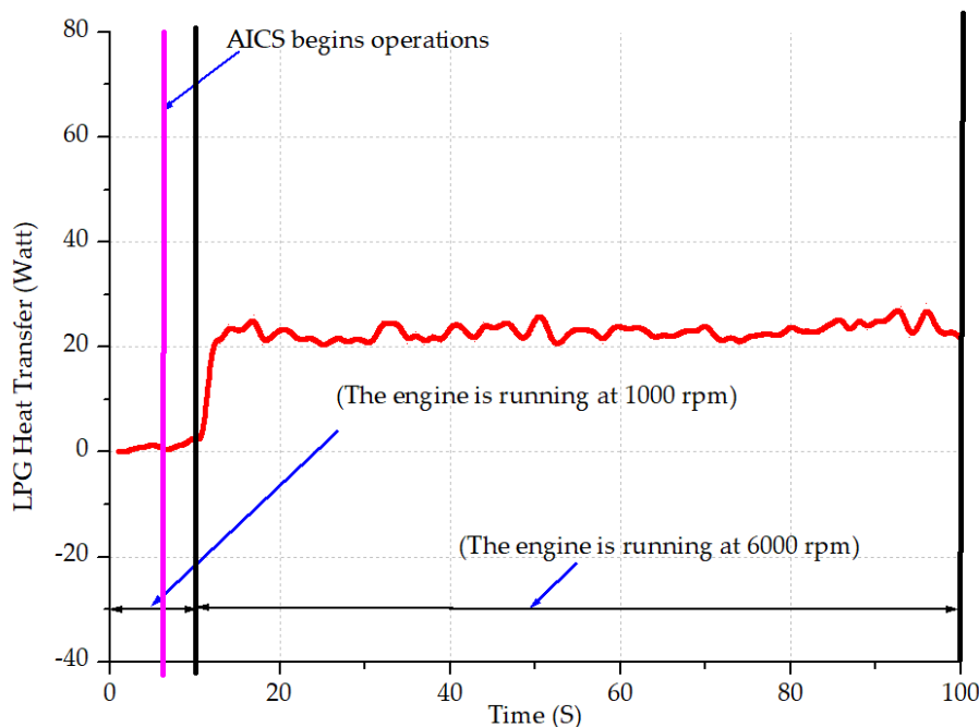
Fig. 13. Heat transfer characteristics of LPG
