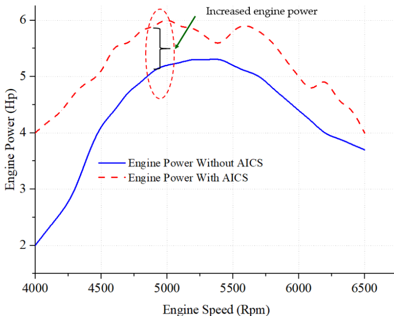
Fig. 5. Increased engine power when the ambient air temperature is hot
