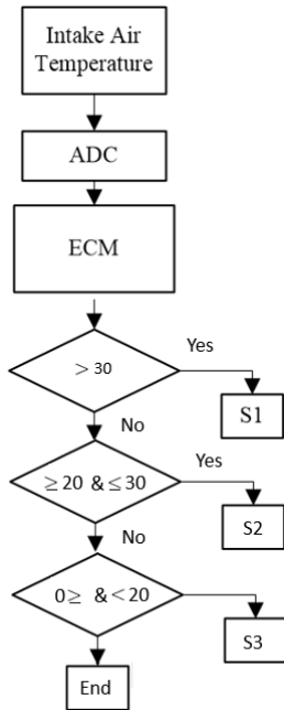
Fig. 3. Control system algorithm
