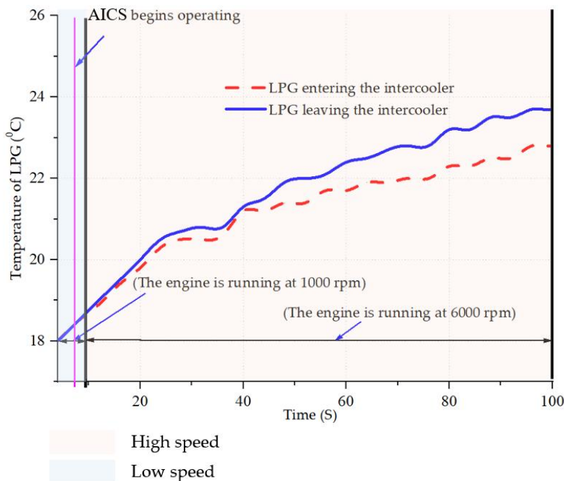
Fig. 11. Changes in the temperature of LPG entering the LPG engine
