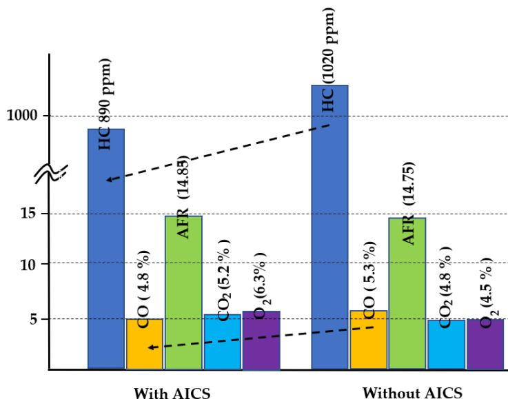
Fig. 4. Changes in LPG engine emission reduction
