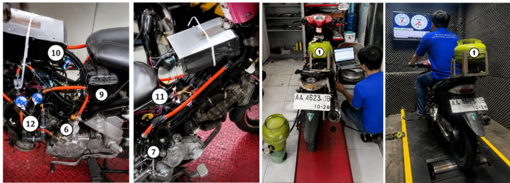
Fig. 1. Settings of AICS
