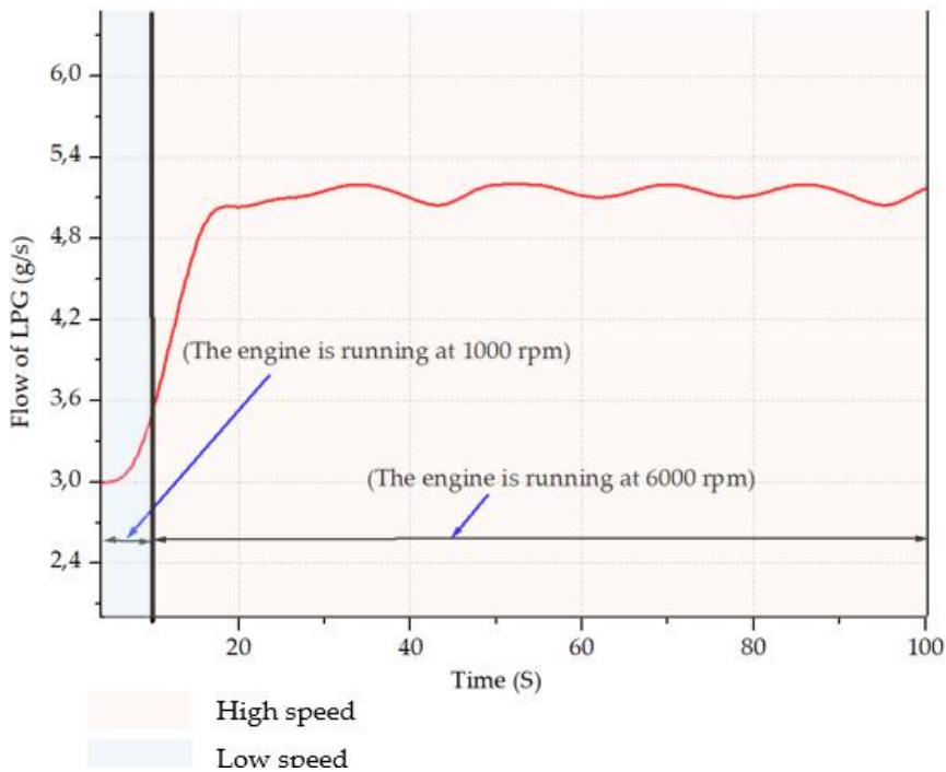
Figure 8. LPG flow dynamics
