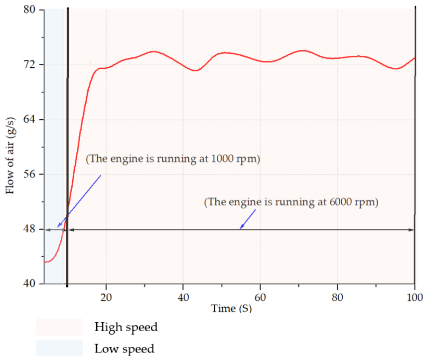
Fig. 9. Air flow dynamics
