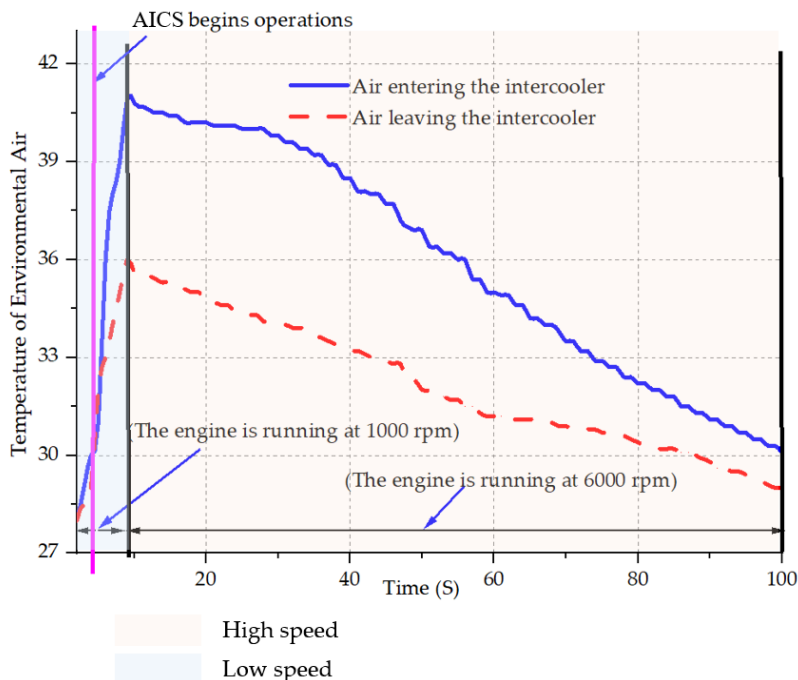
Fig. 10. Changes in the air entering the LPG engine
