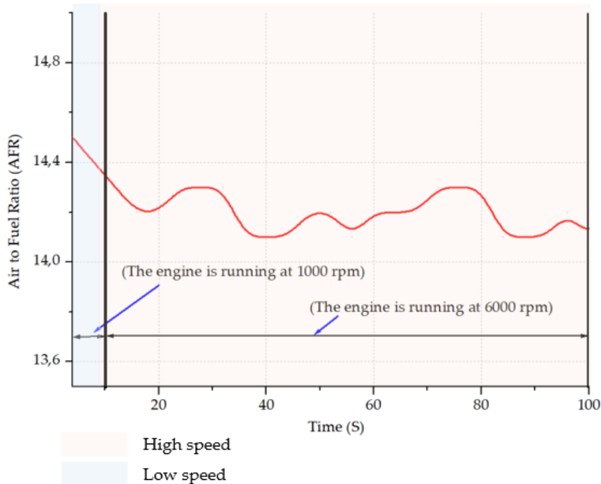
Fig. 7. Changes to the AFR of the LPG engine
