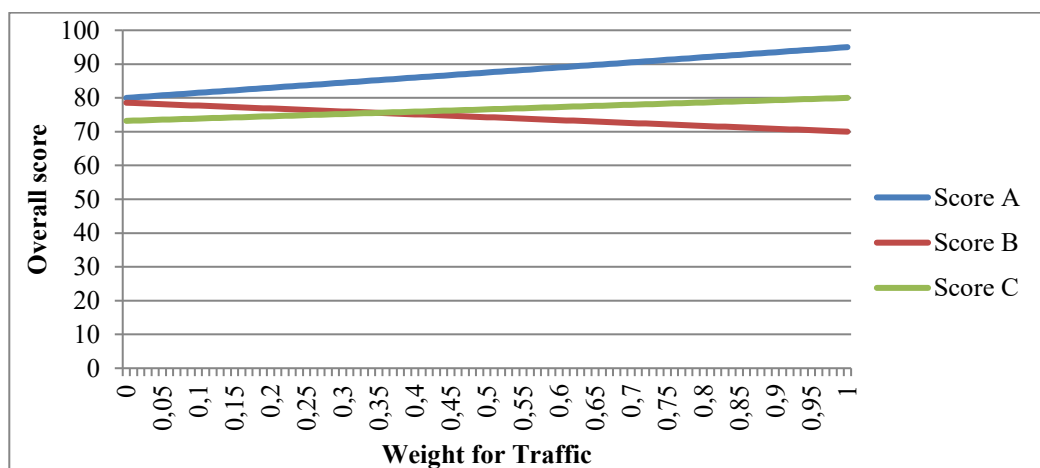
Fig. 2. Scores vs weight for Traffic
