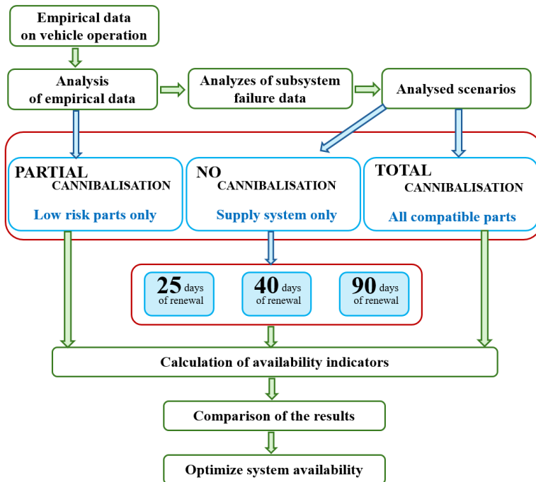
Fig. 2. Cannibalisation-based renewal scenarios: total cannibalisation, partial cannibalisation, and no cannibalisation
