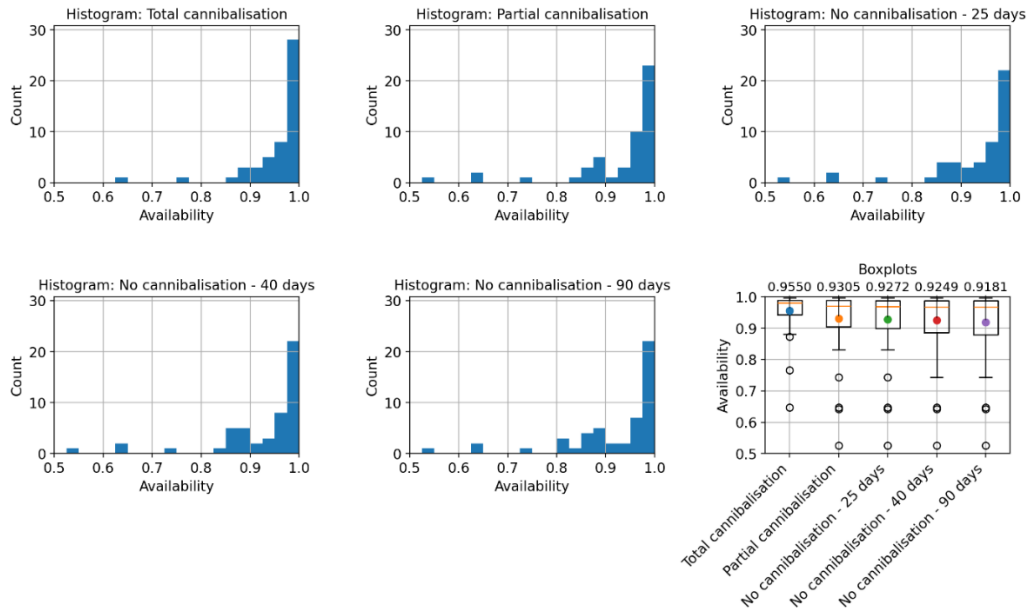
Fig. 9. Distributions of the availability coefficient for individual scenarios
