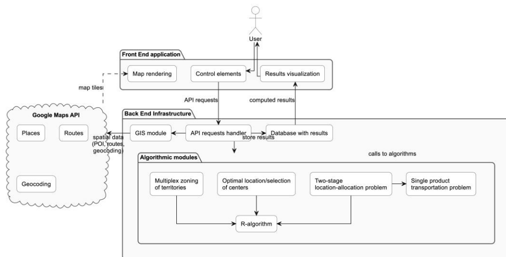
Fig. 1. Software Application Diagram
