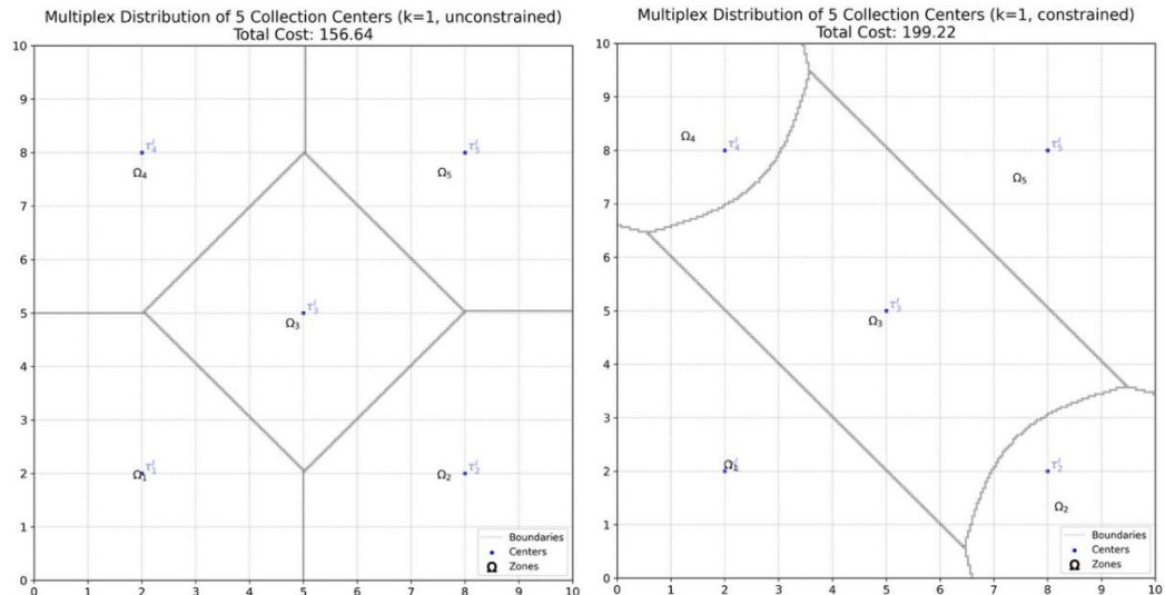
Fig. 4. Accounting for limited capacities of logistics centers: left – zoning without capacity constraints; right – zoning with limited capacities of two centers
