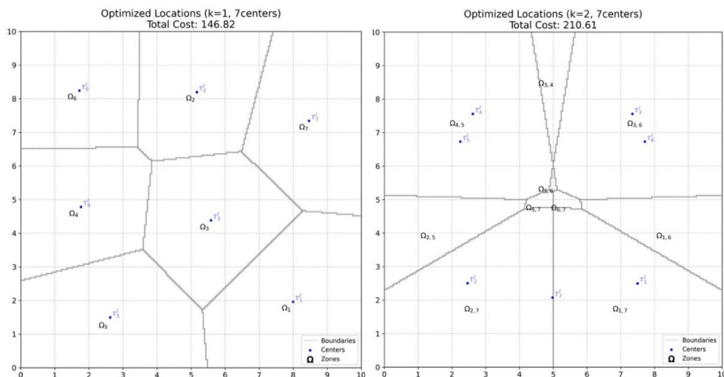
Fig. 3. Optimal location of logistics centers and determination of service zones: left – monopolistic servicing ( k = 1 ); right – duplex coverage ( k = 2 )
