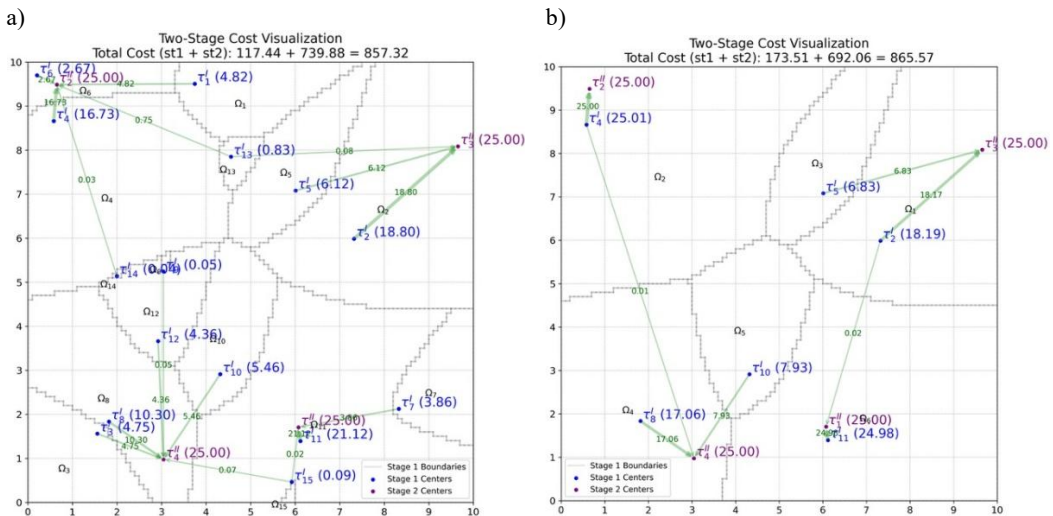
Fig. 2. Two-stage distribution of resources continuously distributed over a square area: a) optimal solution of the problem; b) result of applying the improvement procedure
