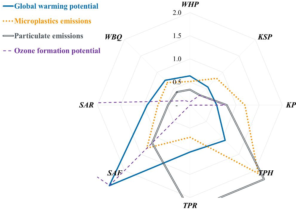
Fig. 3. Comparison of the key properties relative to the average values of each property assumed as 1.0 (assumed periodic renewals of 1.0 m 2 marked surface with the same materials at ½ of physical service life for 20.0 million vehicle passes).
