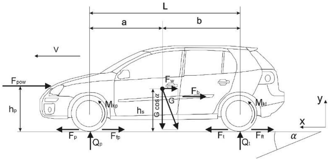
Fig. 4. A system of forces and moments acting on a moving vehicle: Q_t, Q_p – forces of ground response to driving wheels, F_t, F_p – wheel driving forces, F_f, F_{fp} – rolling resistance forces, G – vehicle weight, F_w – grade resistance force, F_b – inertial force, F_{aero} – air resistance force, L – distance between driving wheel axles, a, b – distances of the wheel axles from the vehicle centre of mass, h_p – height of the resultant air resistance force application, h_s – height of the vehicle centre of mass position.
