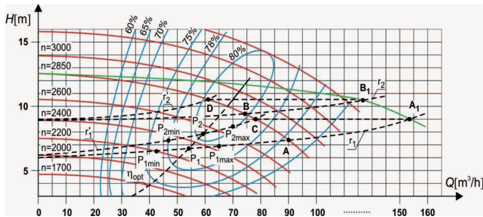
Fig. 7. Analysis of a sewage pumping plant's operation on the basis of the pump's iso-efficiency curve
