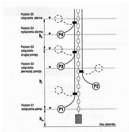
Fig. 2. Control levels of pumping plant's operation; P1 – dry operation sensor, P2, P3 – operation of pump one and two, P4 – alarm sensor [6]
