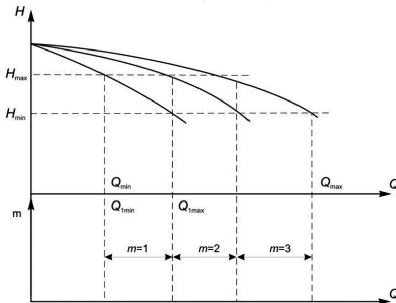
Fig. 3. Flow characteristic of a unit comprising m pumps
