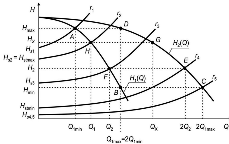
Fig. 4. Flow characteristics of a pump H_1(Q) and of two pumps in parallel H_2(Q)
