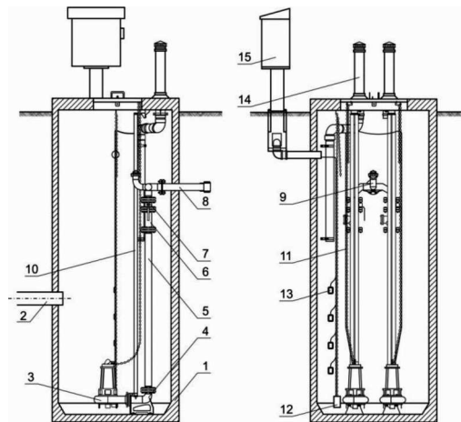
Fig. 1. Rainwater pumping plant made of polymer concrete PB, concrete BT or prestressed concrete BS; 1 – reservoir, 2 – duct for incoming sewage, 3 – immersion pump, 4 – coupling foot, 5 – pumping pipeline, 6 – check valve, 7 – cut-off valve, 8 – sewage disposal pipe, 9 – installation flushing connection, 10 – pipe guides, 11 – chains for lowering and lifting of pumps, 12 – weighted chain, 13 – floating switch, 14 – venting installation, 15 – control cabinet [6]
