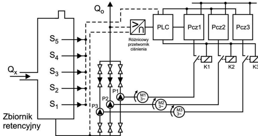
Fig. 8. A piping and instrumentation diagram for a variable speed controlled pumping plant
