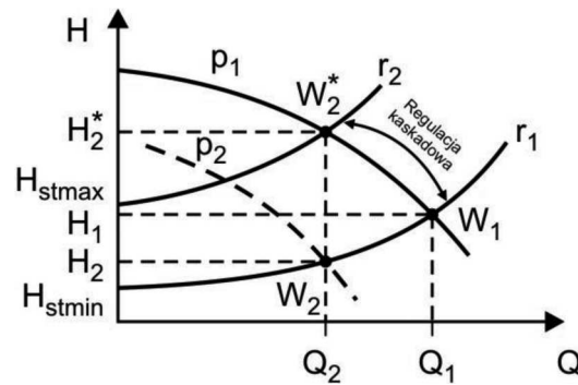
Fig. 5. Flow characteristic of a pump p_1 relative to a reference curve r_1 of a pumping system
