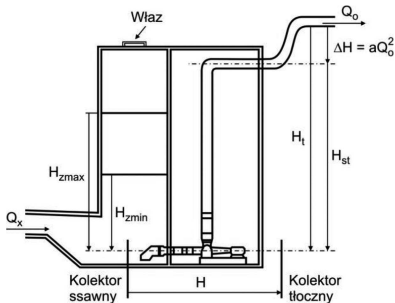
Fig. 6. A sample distribution of head across a sewage pumping plant
