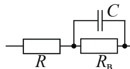
Fig. 4. Capacitive storage replacement scheme
