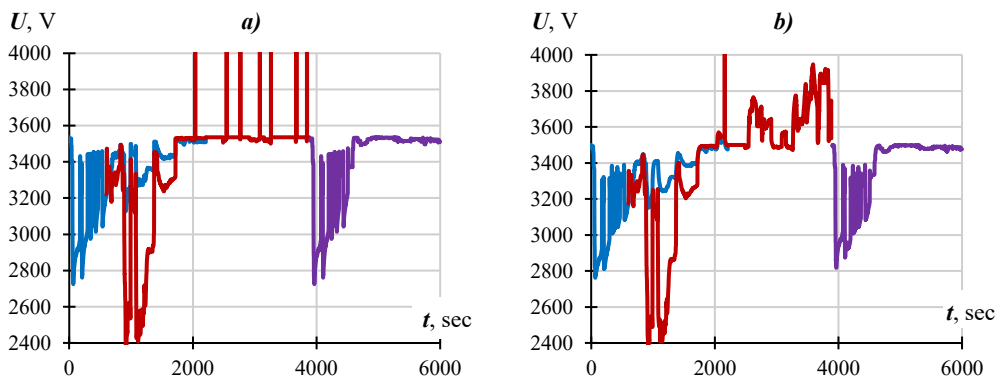
Fig. 14. Current collector voltages of electric locomotives in different operation modes of the traction substation equipment: a - a rectifier without a SU; b - an inverter with a controlled SU
