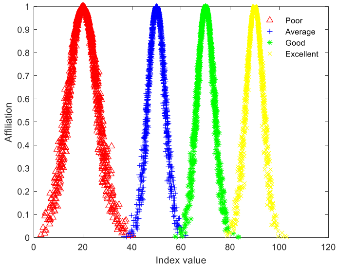
Fig. 5. Cloud drop diagram of non-cash utilization rate of public transit
