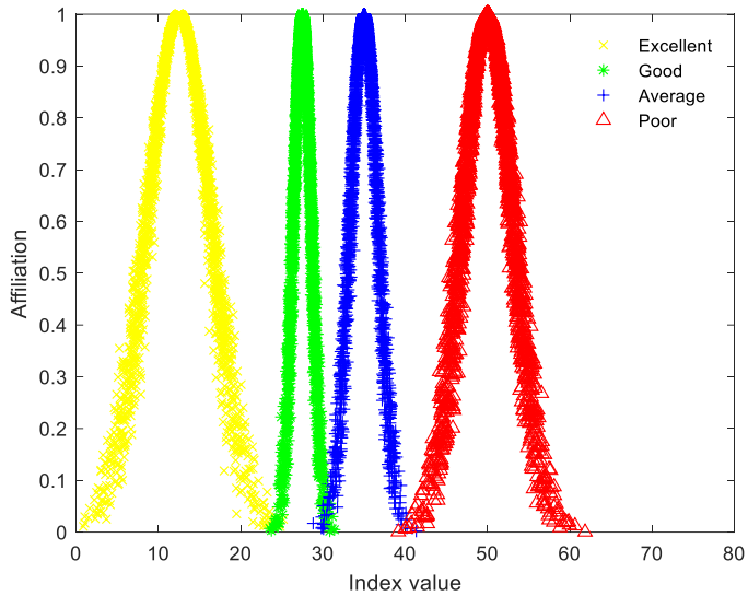
Fig. 4. Cloud drop diagram of average travel time consumption of passengers
