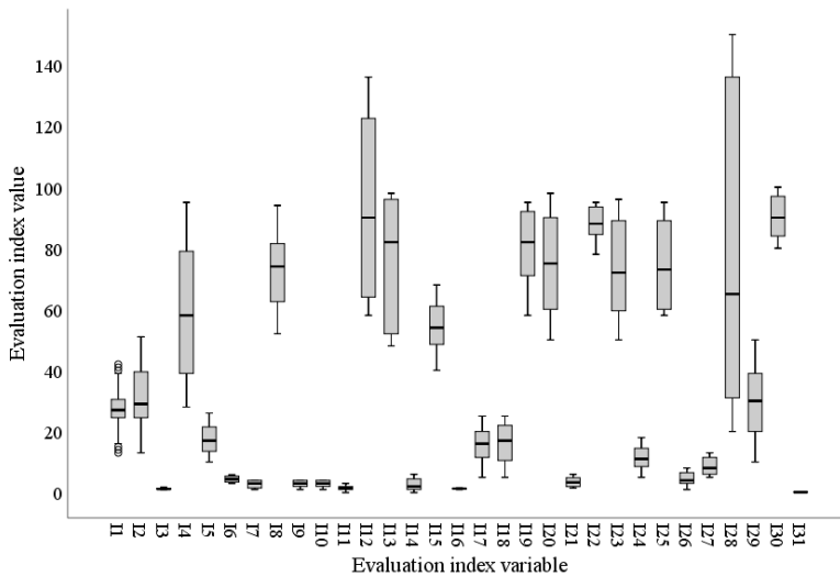
Fig. 3. Boxplot of each evaluation index
