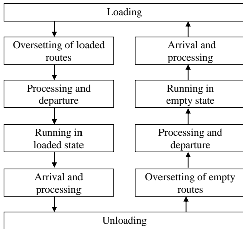
Fig. 3. Schematic diagram of the simulation model of car traffic with grain
