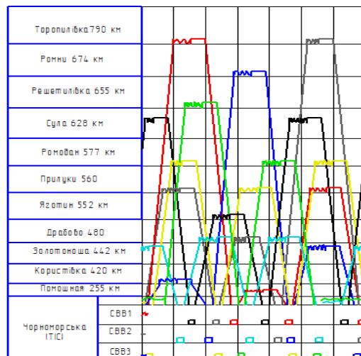
Fig. 4. Diagram of the grain routes
